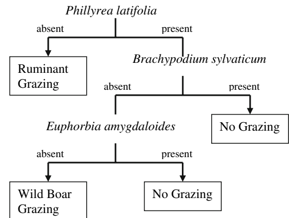
Fig. 1 Classification tree of the grazing regimes (ruminant, boar and no-grazing) on the basis of indicator plants. Each “leaf” is labelled according to presence-absence of the species Phillyrea latifolia , Brachypodium sylvaticum and Euphorbia amygdaloides in the above-ground vegetation. The misclassification error was minor (12%)
